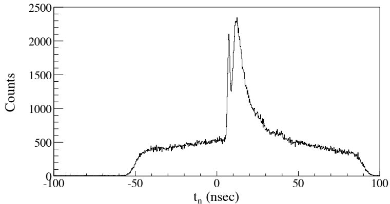
Figure 7-2: The time of flight of the product neutron from LH 2 target to the detector for \theta_p = 12^\circ , \theta_n = 24^\circ , T_{\text{beam}} = 500 \pm 25 MeV.
